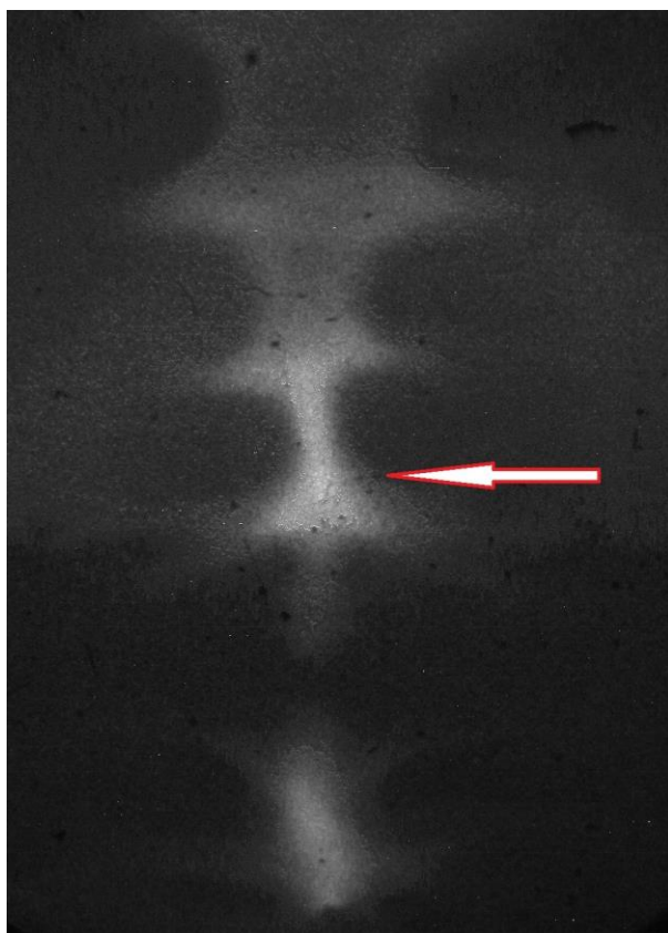
Figure 2. Our smallest plasmoid yet, in formation. The plasmoid is forming at the narrowest “waist” of this image, which is 1 cm across. The waist is only 200 microns in radius. The black specks are defects in the ICCD imaging device.
