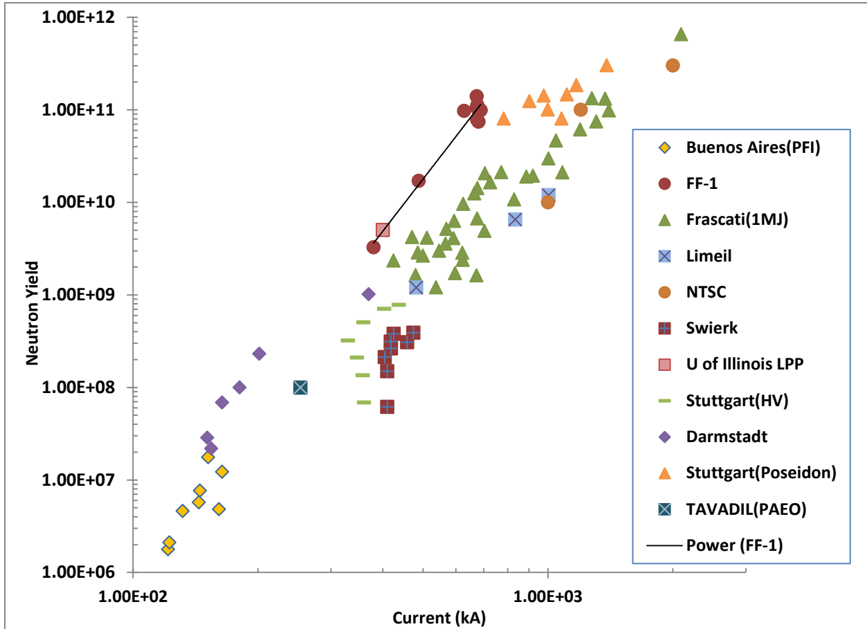
Figure 6. FF-1 SPT results, filled circles on line, fall above the historic trend line of DPF results. Data is from M. Milanese and J. Pouzo [31], except for U of Illinois and FF-1. Line is power-law fit to FF-1 data.
