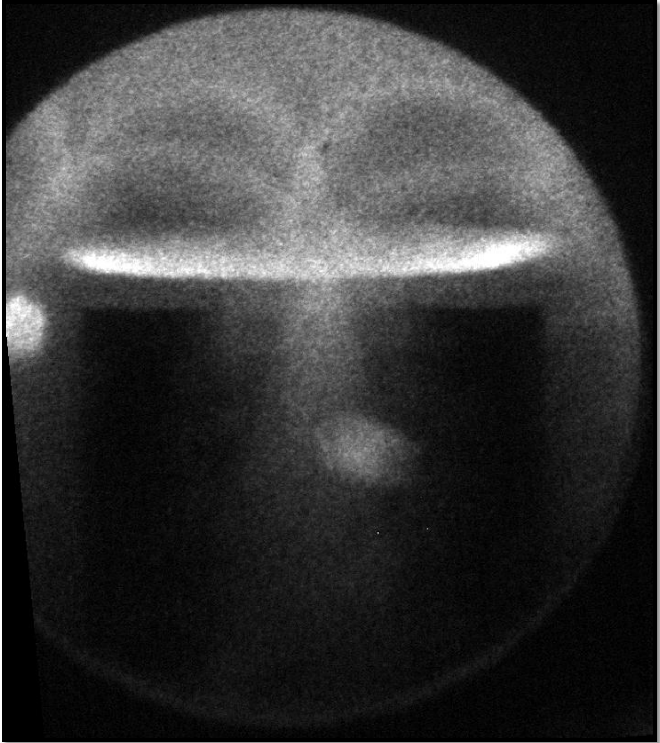
Figure 5. ICCD image of end of anode at 225 ns before pinch, exposure time 0.2 ns. Note the convergence of the filaments at this time on the axis of the anode. The circle is the viewing window and the bright horizontal ellipse is the hole in the anode.
