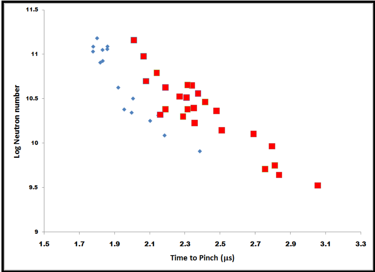
Figure 2. Log neutron yield vs time to pinch. The small dots are shots at 10 torr fill pressure while the large ones are at 18-24 torr. Error bars are omitted for clarity and are 0.1 for log yield and extremely small—less than 5 ns—for time. Quarter-cycle time is 1.8 \mu\text{s} .
