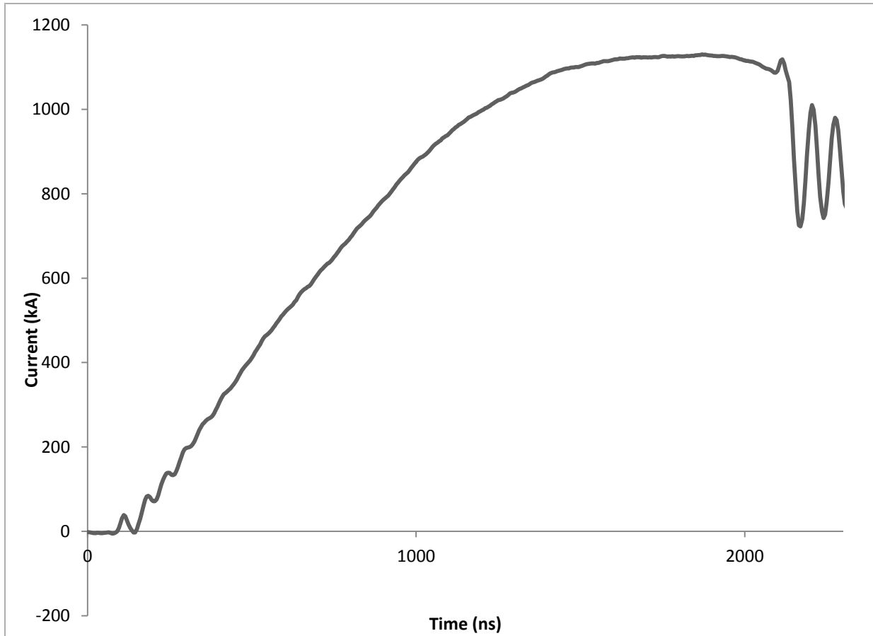
Figure 3. Current vs time, shot 10011002, an LPT, with pinch process starting with negative dI/dt . Note the small bump in current before the pinch.
