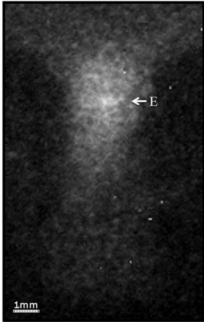
Fig. 4 Shot 102603, 55 ns before pinch peak. Kink has started to condense into the very dense plasmoid at [E].
