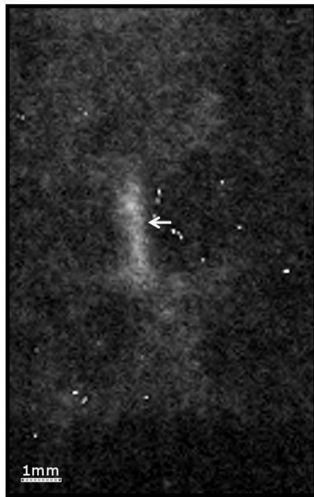
Fig. 2 In this ICCD 200 ps exposure of Shot 102604, 92 ns before pinch peak, the dense plasma pinch column is condensed, but just starting to form a helix.
