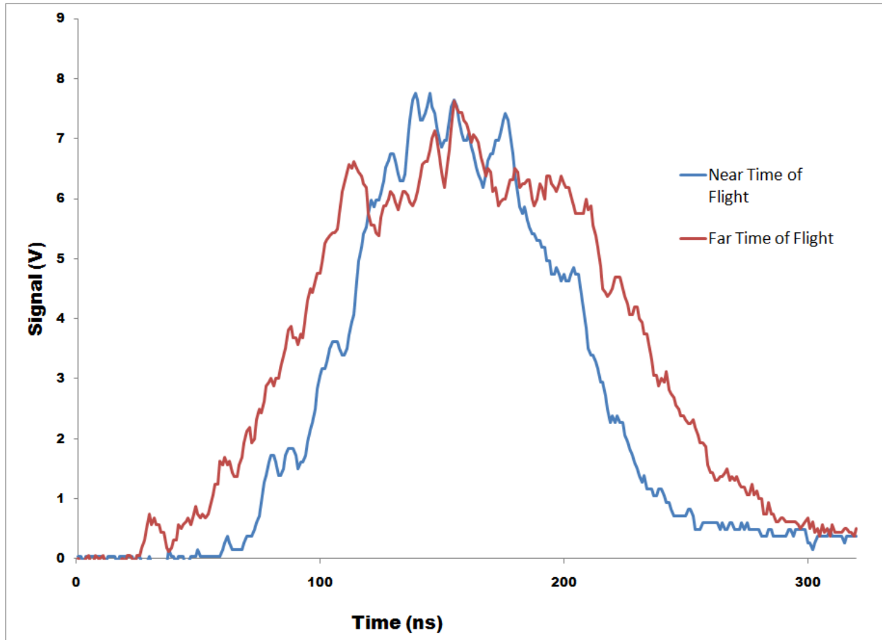
Fig. 1 These signals are from the 11-meter (near-blue) and 17-meter (far-red) neutron detectors for shot 9301002. The greater spread in the time in the signals at 17 meters was used to calculate that the ions producing these neutrons had energies of between 160 and 220 keV.
