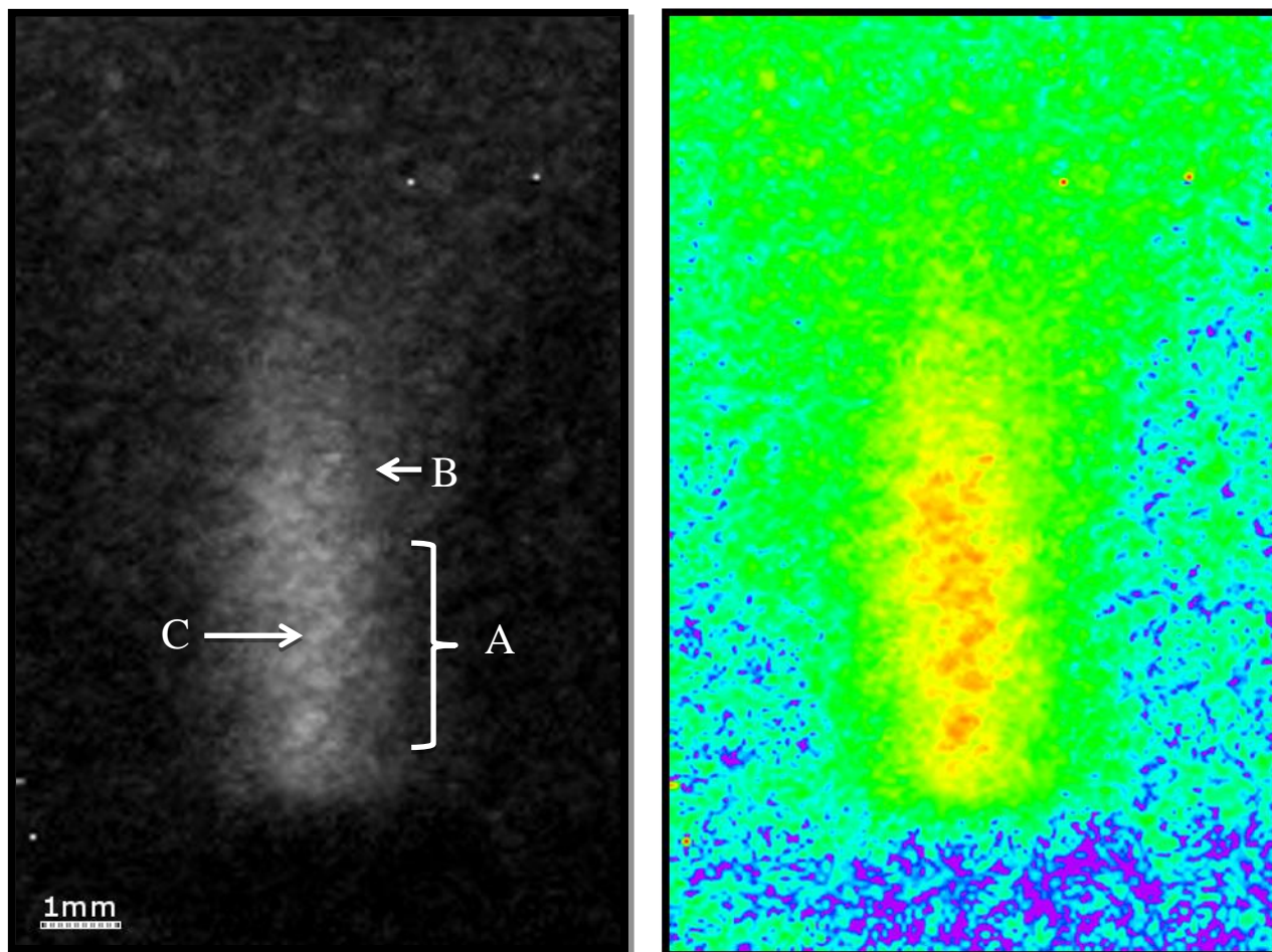
Fig. 3 The axial condensation from shot 101402, 200 ps exposure, 85 ns before pinch peak. Bright filament [C] is about 240 microns in diameter. The helical filament has started to kink—note the formation of kink [B] at top of helix. False color image at right has brightest radiation as red, dimmest as blue.
