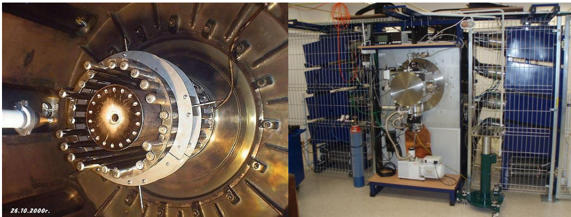
Figure 1. The PF-1000 (left) and the PF-24 (right) will join the FF-1 in experiments with pB11 fuel in 2018.
