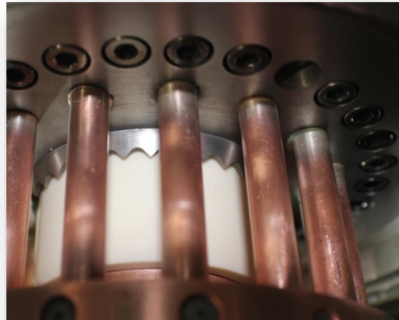
The saw teeth above are one solid piece with the tungsten base, eliminating a current contact that had caused arcing. The teeth concentrate electric fields to enhance filamentation in the plasma sheath that extends outward to the copper rods.
