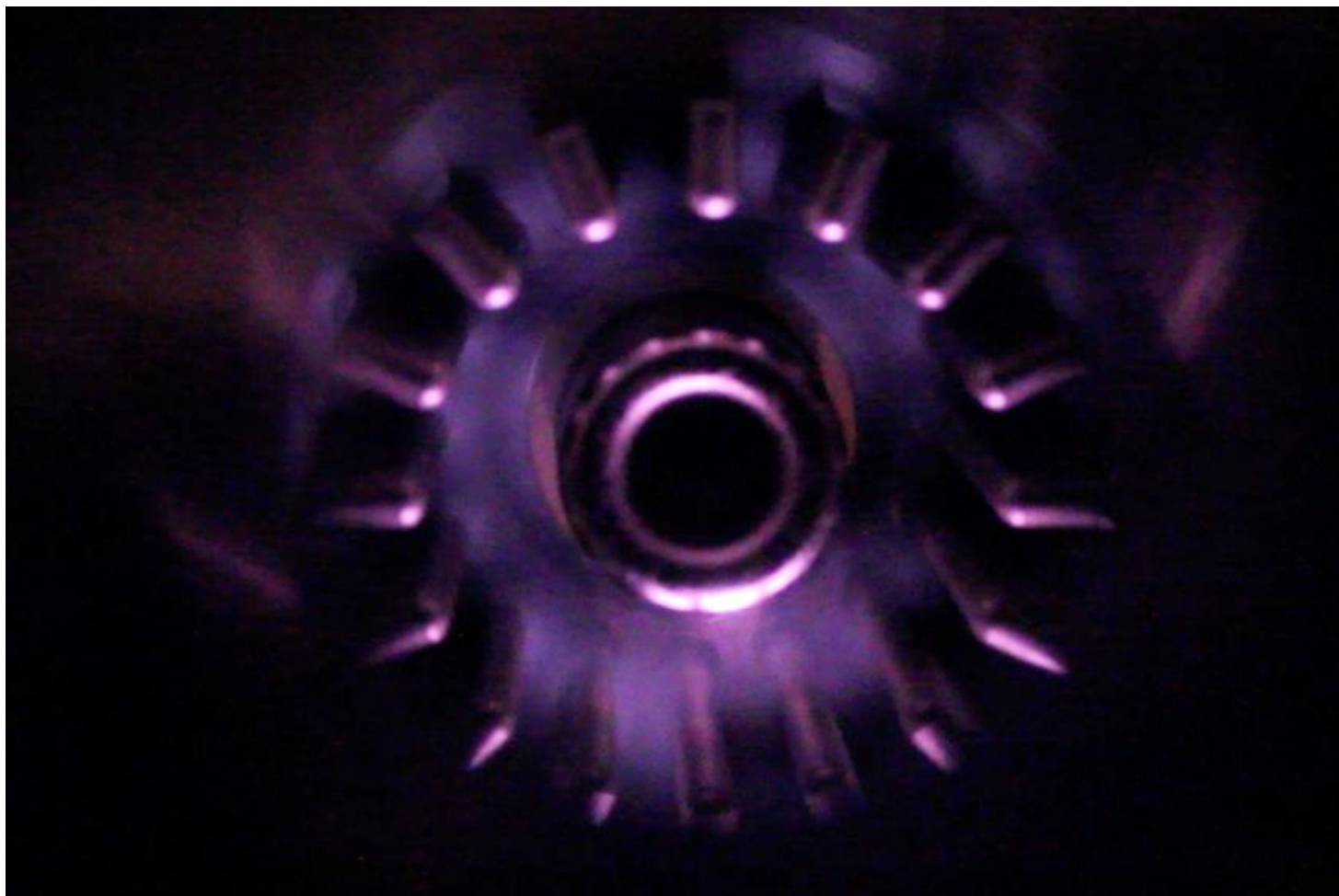
Fig. 2 Microwaves generate the hot glowing plasma between the anode (inner cylinder) and cathode (outer vanes), which removes oxygen from tungsten oxides. But we need to make the coverage of the plasma more even to get all the oxides off.
