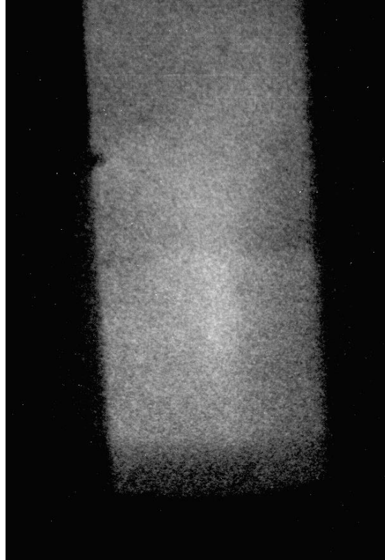
Fig. 3 ICCD image of shot 4, Jan 31 2017, exposure time 200 ns. The image shows the 1-cm wide region visible between two adjacent cathode vanes, on the axis of the device. The image is inverted, with the end of the anode at the bottom of the image. The bright central region is the pinch, containing the plasmoid, which is considerably blurred by its rapid vertical motion during the exposure. We expect soon to get much sharper images with shorter exposures.
